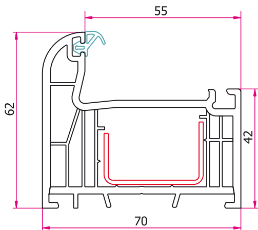
Toc TP6101 - standard Toc TP6101 - Eco Telaio TP6101- standard Telaio TP6101- Eco Tok TP6101 - Standard Tok TP6101 - Eco
